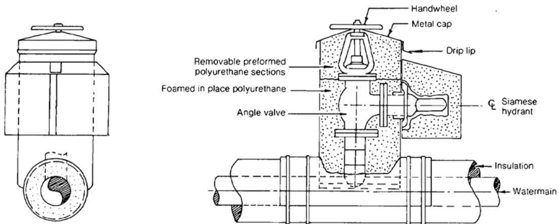
Figure 9 Above-ground hydrant
