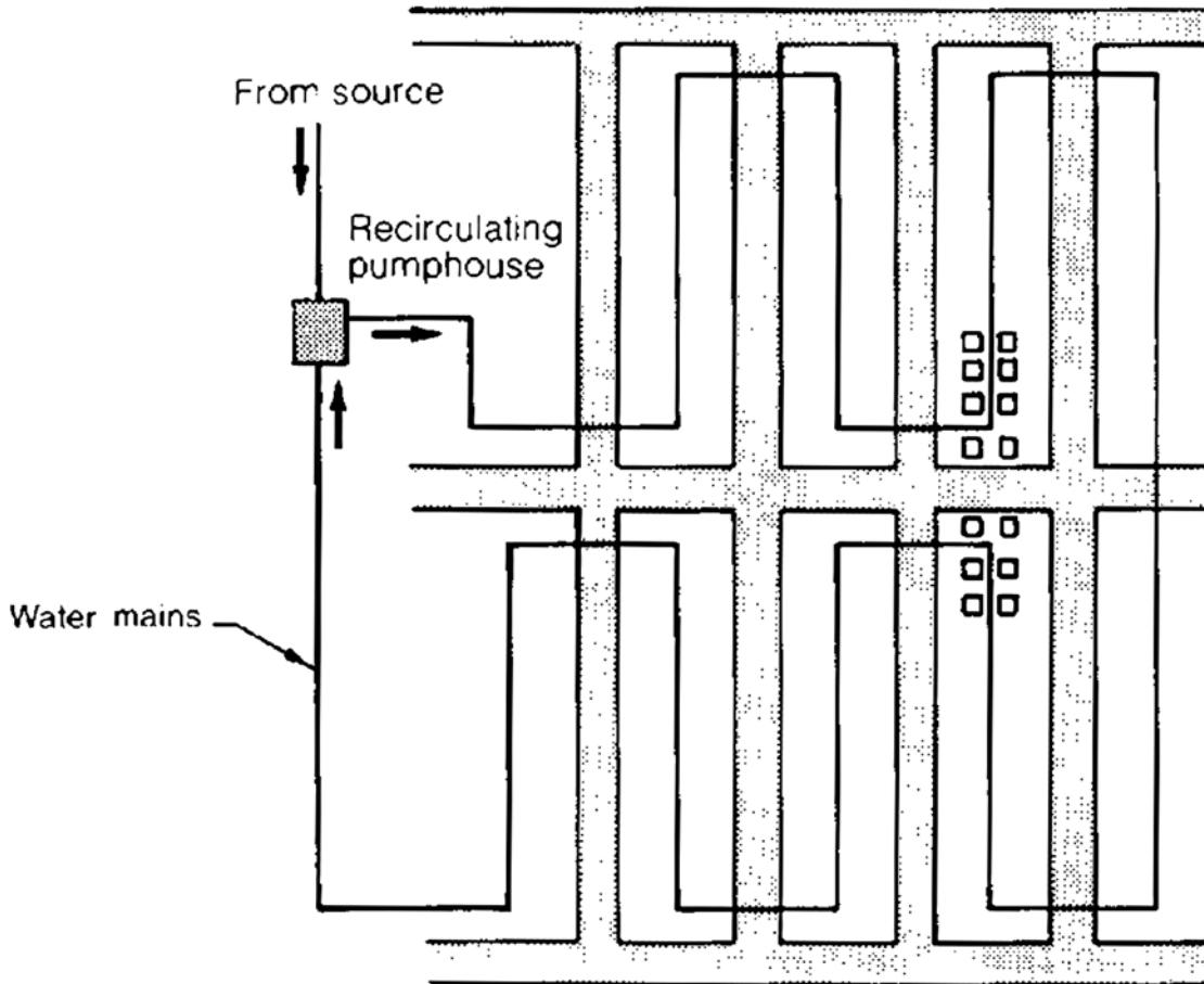
Figure 1 Layout and location of mains for single pipe recirculation
